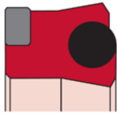
Seal Profile: DK104R
