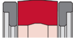
Seal Profile: DK117
