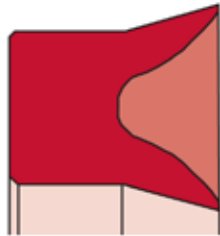
Seal Profile: DS139
